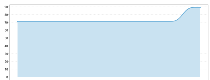
Security Hotspots
