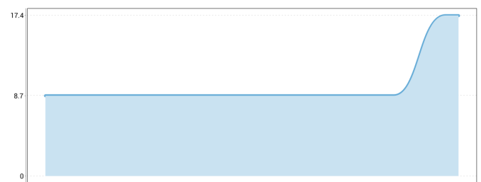
Duplicated Lines (%)
