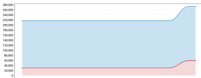
Duplications (Lines of code / Duplicated lines)
